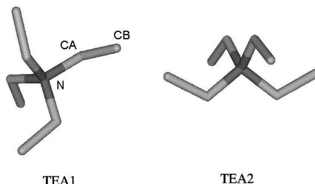
Fig. 2. The pyramidal and quasi-planar conformations of TEA.
